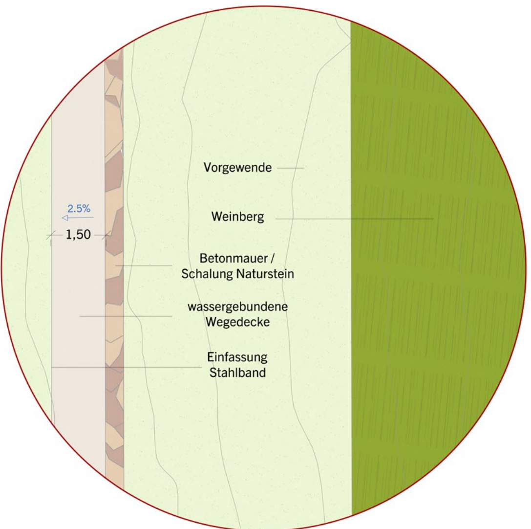
Regeldetail A
